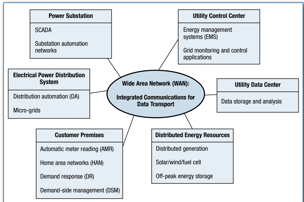
Figure 2: A utility WAN under Smart Grid applications is required to handle more robust data transport.
